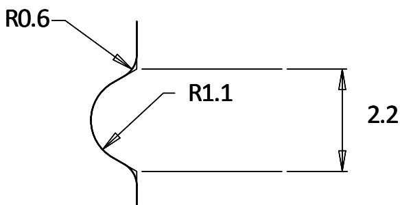
THREAD DETAIL
